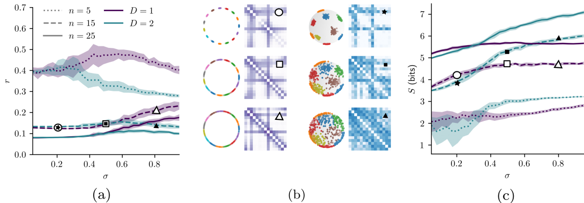
Figure 3.7 – (a) Stable rank to dimension ratio and (c) Shannon entropy of community block matrices in \mathbb{S}^1 and \mathbb{S}^2 , when increasing the angular dispersion of nodes. The center panel (b) illustrates examples of angular coordinates and block matrices with \sigma \in \{0.2, 0.5, 0.8\} for D = 1 (purple matrices) and D = 2 (blue matrices) with corresponding values of stable rank and indicated with symbols on (a) and (c). All the graphs have \beta/D = 3.5 and a Pareto expected degree distribution with average degree of 4.0 and \gamma = 2.5 .
