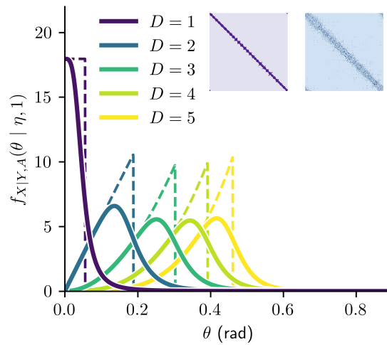
Figure 3.3 – Probability density functions of angular distance between connected nodes in the \mathbb{S}^D model given by Eq. (3.17), for N = 1000 nodes, with \kappa = \kappa' = 10.0 and \beta/D = 3.5 . For D = 1 , the maximum is at \theta = 0 , as depicted in the purple example connectivity matrix where the dark diagonal line illustrates all of the connection probability concentrated to very small angular distances. In D \geq 2 , this is relaxed, as shown by the blue curve and connectivity matrix. The dashed lines show the \beta \rightarrow \infty limit. Matrices represent a \mathbb{S}^D connection probability matrix for D = 1 (left) and D = 2 (right), \kappa_i = 10.0 for all nodes i , ordered according to the polar coordinates.
