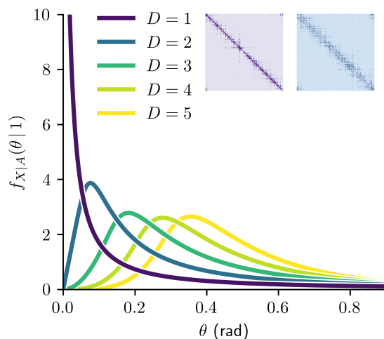
Figure 3.4 – Probability density functions of angular distance between connected nodes in the \mathbb{S}^D model given by Eq. (3.23), for N = 1000 nodes, \beta/D = 3.5 and with a Pareto latent degree distribution with \bar{k} = 10.0 and exponent \gamma = 2.5 . Matrices represent a \mathbb{S}^D connection probability matrix, for D = 1 (left) and D = 2 (right), ordered using the polar coordinates of the nodes.
