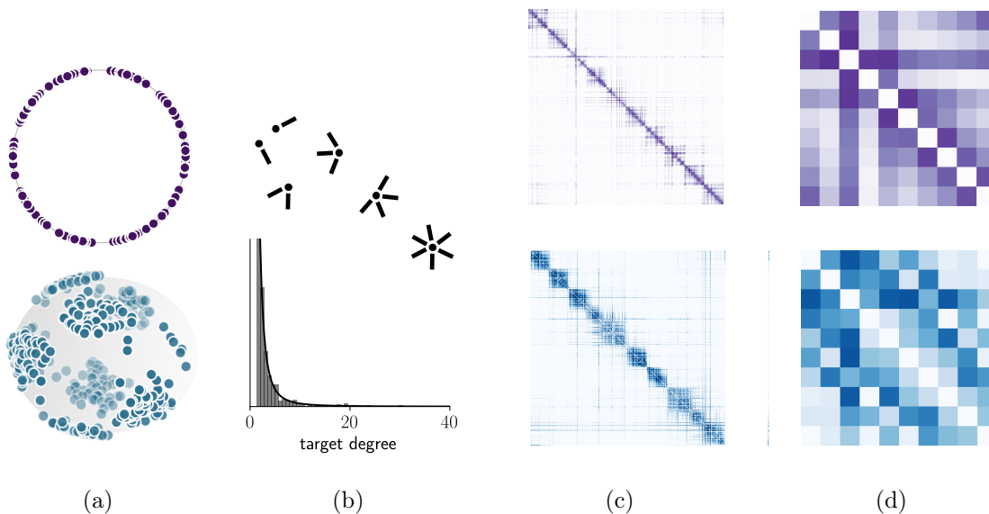
Figure 3.6 – Example of sampling hyperbolic random graphs with angular community structure in \mathbb{S}^1 and \mathbb{S}^2 . Angular coordinates (a) are used to optimize latent degrees such that a given expected degree distribution (b) is achieved. The random graphs are then fully specified by Eq. (3.5), which is illustrated in (c) matrices of connection probabilities between all nodes, ordered with polar coordinates within each community. Those are then coarse-grained into block matrices (d) using Eq. (3.32) to study inter-community interactions in hyperbolic spaces.
