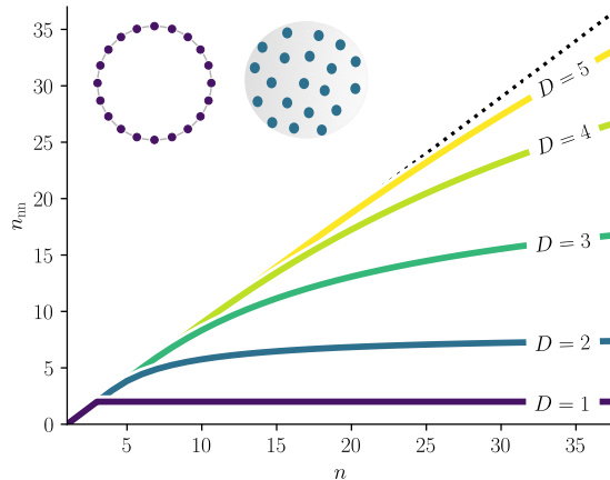
Figure 3.5 – Number of nearest neighbors n_{\text{nn}} given by Eq. (3.26) for D \in \{1, 2, 3, 4, 5\} . The dotted line is at n - 1 , the maximal number of neighbors for n points on S^D . A circle and a sphere are also shown to exemplify neighboring points in D = 1 and D = 2 .
