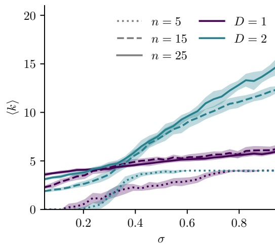
Figure 3.8 – Average community degree \langle k \rangle of hyperbolic random graphs with angular communities sampled in \mathbb{S}^1 and \mathbb{S}^2 . All the graphs have \beta/D = 3.5 and a Pareto expected degree distribution with average degree of 4.0 and \gamma = 2.5 .
